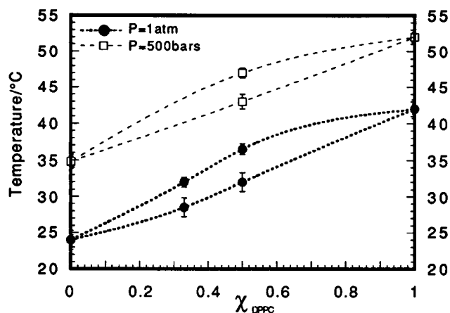
FIGURE 8 Effect of pressure on the thermotropic phase diagram of the DMPC/DPPC lipid mixture. (●) Phase diagram constructed at atmospheric pressure from the lifetime distributions of t -PnA (see preceding paper). (□) Data obtained at 500 bar (see text). At \chi_{DPPC} = 1 and P = 500 bar the temperature value is taken from Chong and Weber, 1983b.
