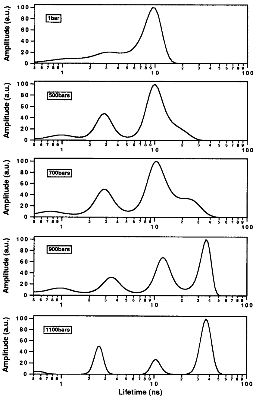
FIGURE 3 Effect of pressure on the lifetime distribution of t -PnA in POPC large unilamellar vesicles at 10^\circ\text{C} .
