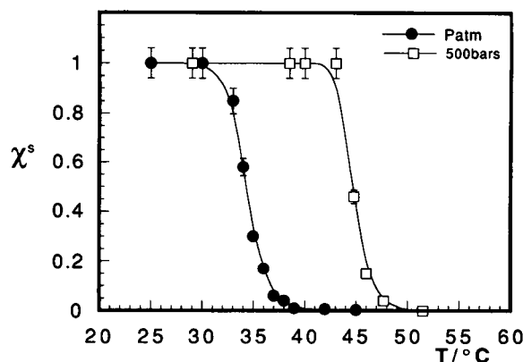
FIGURE 7 Temperature dependence of the gel phase fraction \chi^S of large unilamellar vesicles of an equimolar mixture of DMPC/DPPC at 1atm (●) and at 500bar (□).
